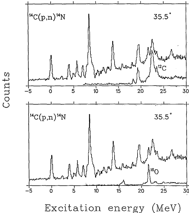
FIG. 2. Excitation-energy spectrum at 35.5^\circ for the ^{14}\text{C}(p,n)^{14}\text{N} reaction at 135 MeV showing the normalized contaminant spectra from the ^{12}\text{C}(p,n)^{12}\text{N} and the ^{16}\text{O}(p,n)^{16}\text{F} reactions.
