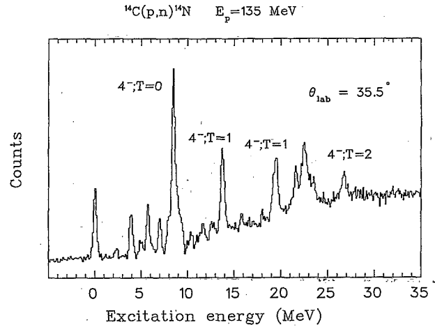
FIG. 3. Excitation-energy spectrum for the ^{14}\text{C}(p,n)^{14}\text{N} reaction at 135 MeV and momentum transfer of about 1.6 fm ^{-1} .
