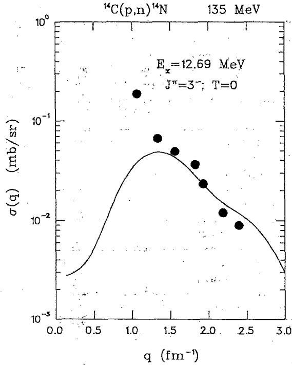
FIG. 10. Differential cross section measured for the 12.69 MeV state in ^{14}\text{N} . The curve shows a DWIA calculation for the 1p_{3/2} \rightarrow 1d_{5/2} transition to the 3^-;0 state.
