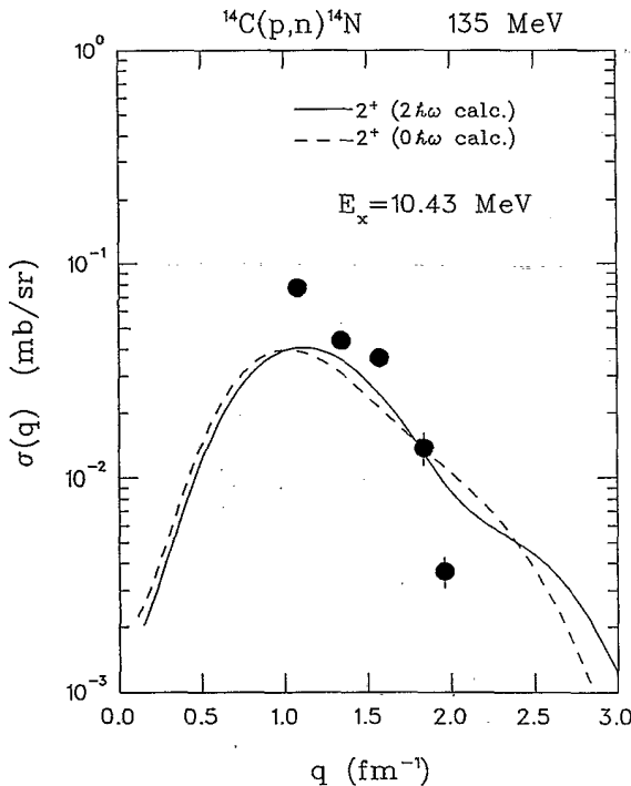
FIG. 8. Differential cross section measured for the 10.43 MeV state in ^{14}\text{N} . The curve shows a DWIA calculation for the transition to the 2^+;1 state employing OBDME's obtained from a shell-model calculation.
